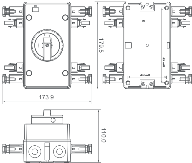
PRODUCT DIMENSIONS (MM)
