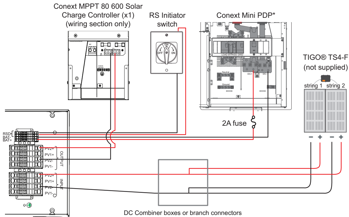
Figure 9 Connection to a single Conext MPPT 80 600 Solar Charge Controller
